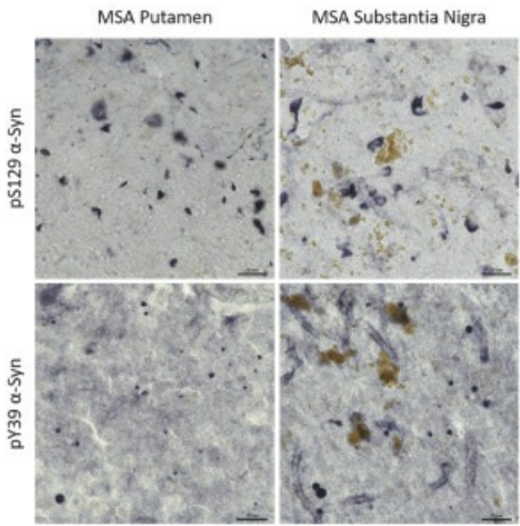
Fig. 12: GICs from human MSA patient brain contain Y39-phosphorylated and S129-phosphorylated alpha-synuclein aggregates. 40 μm coronal sections of human postmortem brain from MSA patients with a diagnosis of “definite MSA” were immunostained using antibodies to detect pathological forms of alpha-synuclein, phosphorylated at Ser 129 (pS129 α-Syn) and phosphorylated at Tyr 39 (pY39 α-Syn). Putamenal sections (left column) show positive staining of glial cytoplasmic inclusions (GICs, black/blue punctate staining) throughout the entire putamen with both pS129 and pY39. Nigral sections (second column from left) show positive staining of GICs (black/blue punctate staining) throughout the substantia nigra, in close vicinity to neuromelanin positive neurons (yellow-brown staining). Scale bars = 25 μm.
